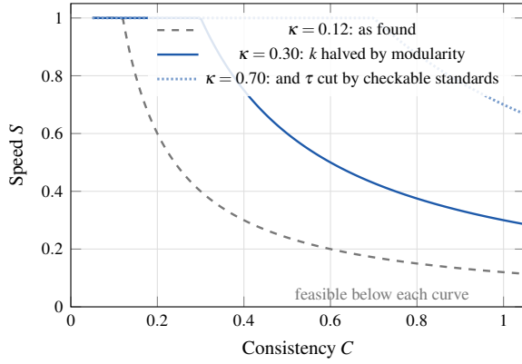
Figure 2. The frontier S \leq \kappa/C at full autonomy ( A = 1 ). Each curve is the most speed an enterprise can have for a given consistency; points above it are infeasible. Lowering interdependence ( k ) and reconciliation latency ( \tau ) moves the frontier outward but never to the corner (1, 1) : the trilemma is relaxed, not removed. Values illustrative.
