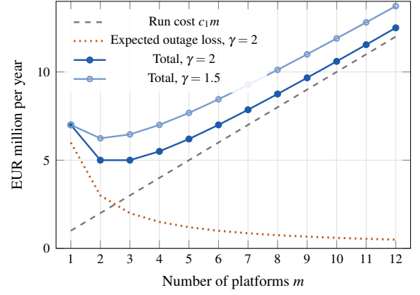
Figure 1. The high-stakes regime of Table 1 ( p = 0.10 , \ell = 60 , c_1 = 1 ). Run cost rises with platforms; expected outage loss falls when the loss is convex; their sum has an interior minimum. With \gamma = 2 the optimum is between two and three platforms and one platform costs EUR 2 million a year more; with \gamma = 1.5 the optimum is two and the premium smaller. With \gamma = 1 the loss line would be flat and one platform optimal.
