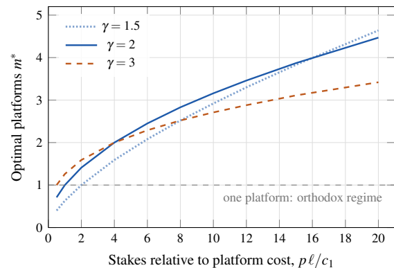
Figure 2. The optimal number of platforms against the stakes ratio p\ell/c_1 , for three convexities. Below a ratio of about one, full standardisation is optimal; above it the optimum rises slowly with the stakes. The curves cross because higher convexity raises the loss from large outages but also the benefit of the first split more than of later ones.
